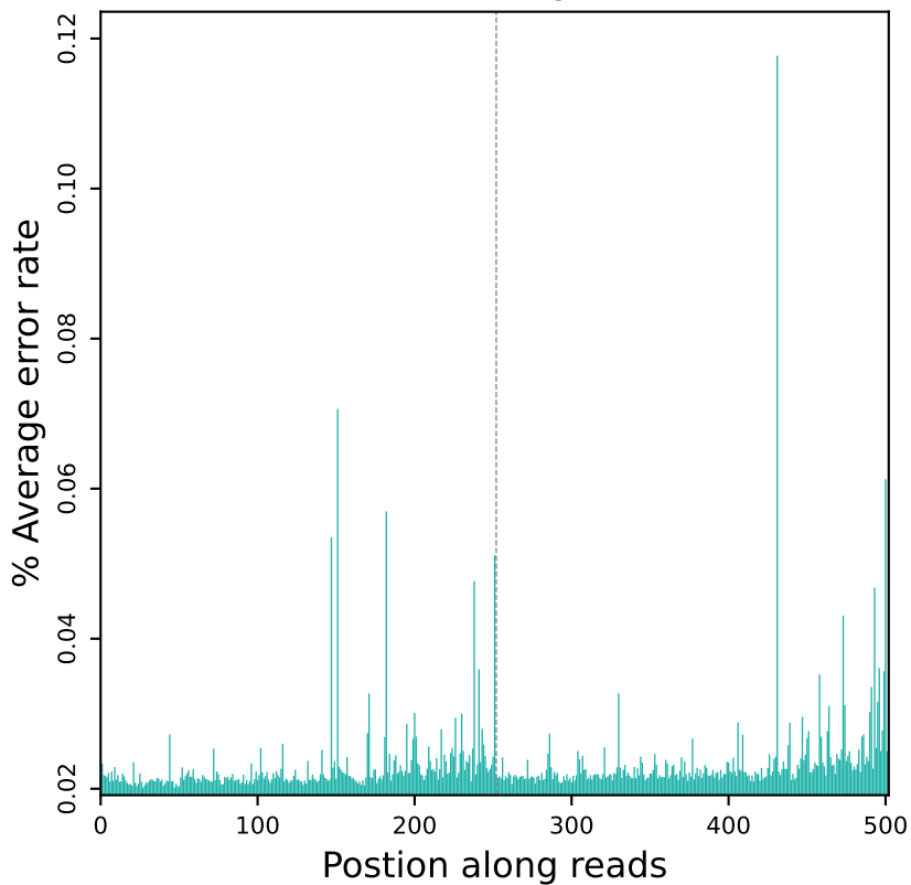
Error rate distribution along reads (R10705)
